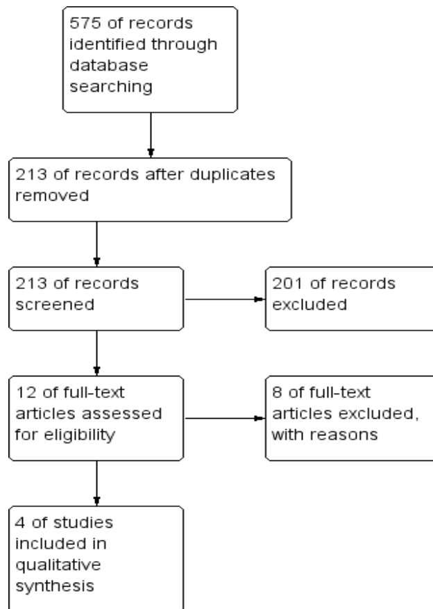
Figure 1. Flow chart of the identifying and retrieving process of studies
